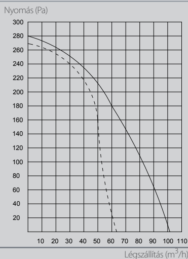
Jelleggörbék
